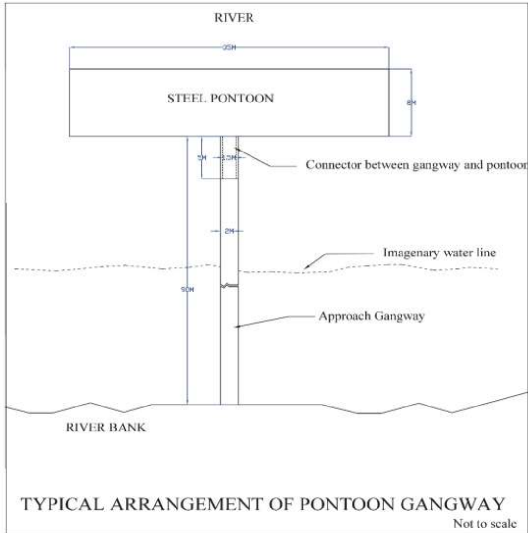
Drawing is indicative only for tendering purpose
