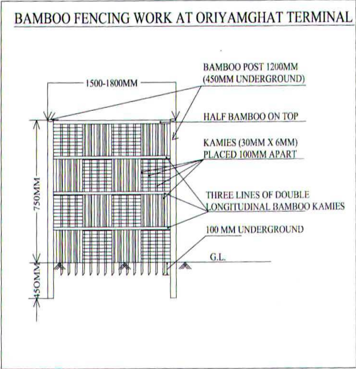
Annexure – IV (TYPICAL DRAWING OF BAMBOO FENCING)
