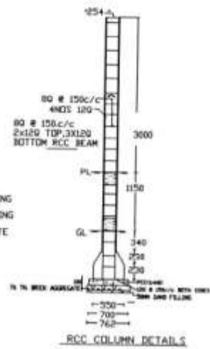
RCC COLUMN DETAILS
