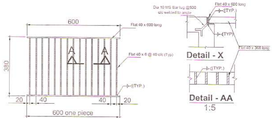
Detail plan of grating 1:10
