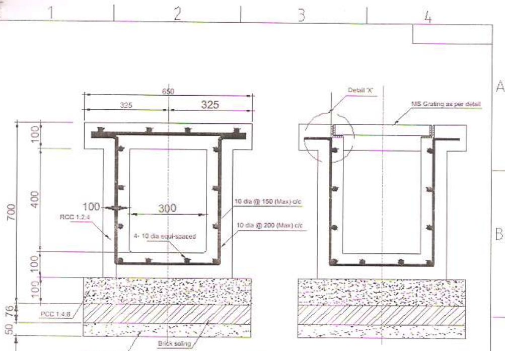
Cross section of drain 1:10
