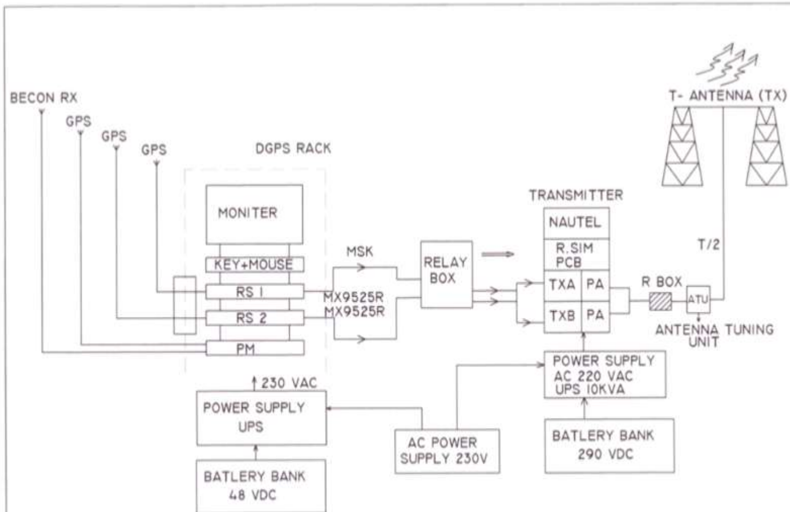
DGPS BHAGALPUR BLOCK DIAGRAM DIFFERENTIAL GLOBAL POSITIONING SYSTEM FREQUENCY = 300 KHZ SERIAL No. - BI99
