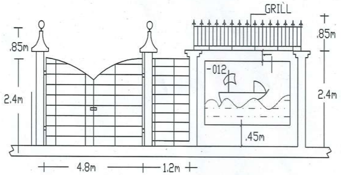
ELEVATION OF GATE AND COMPOUND WALL
