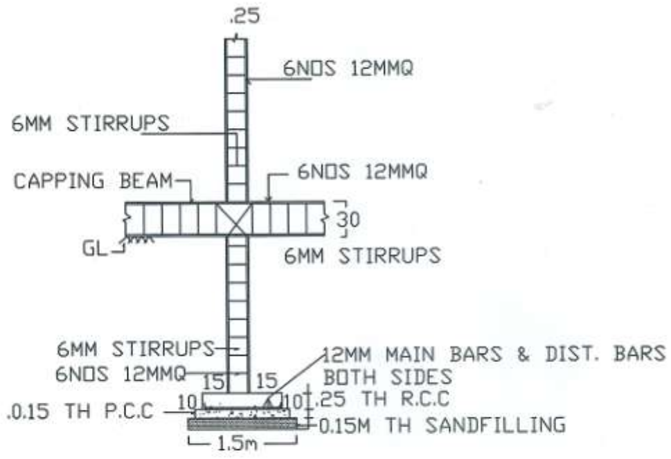
FOUNDATION DETAILS
