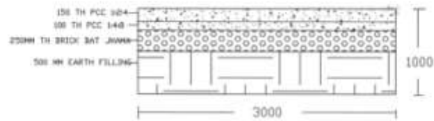
SECTION OF ROAD E-E
