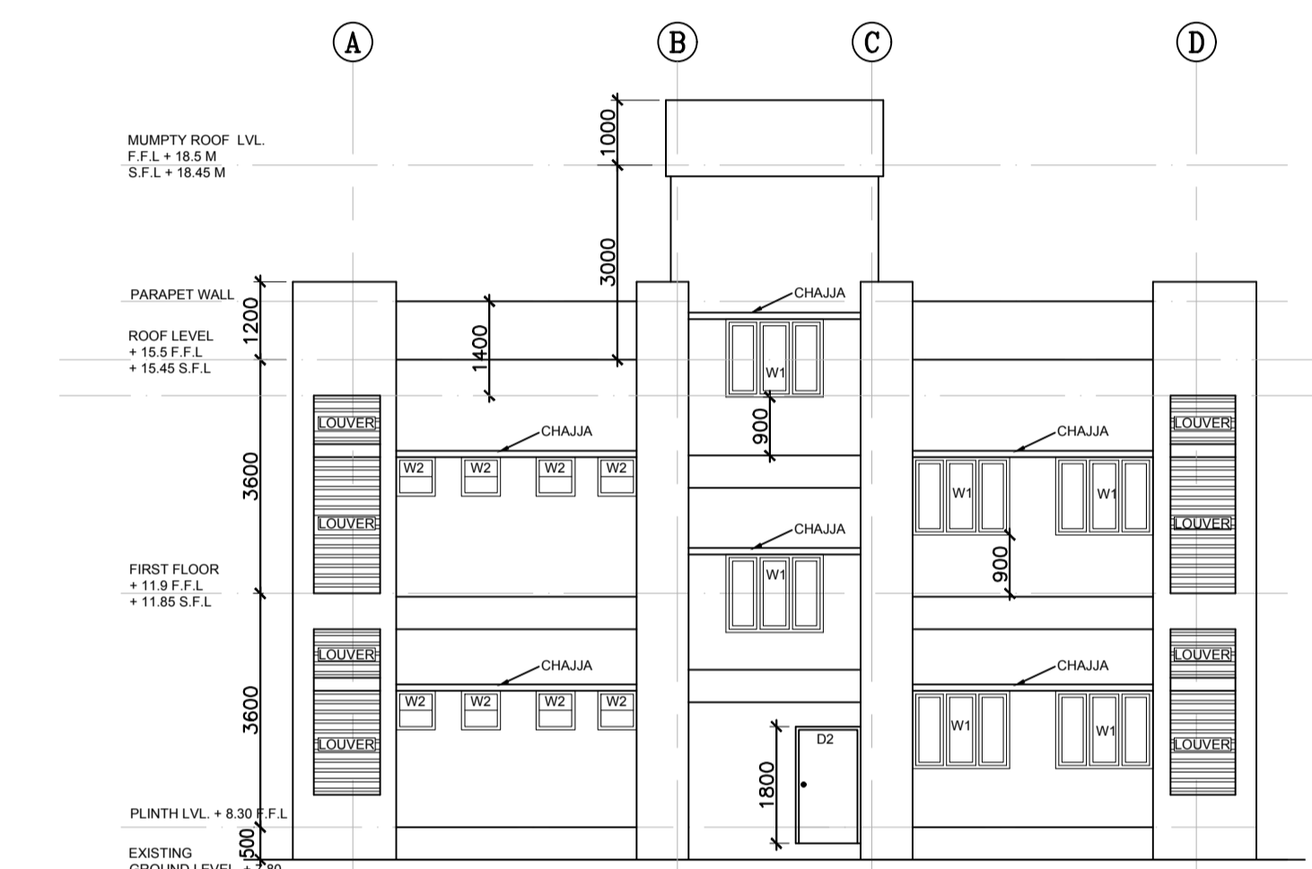
ELEVATION - 4 (SCALE 1:100)
