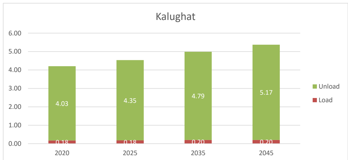
Figure 83: Kalughat Terminal loaded versus unloaded cargo 2020-2045 (million tons)
