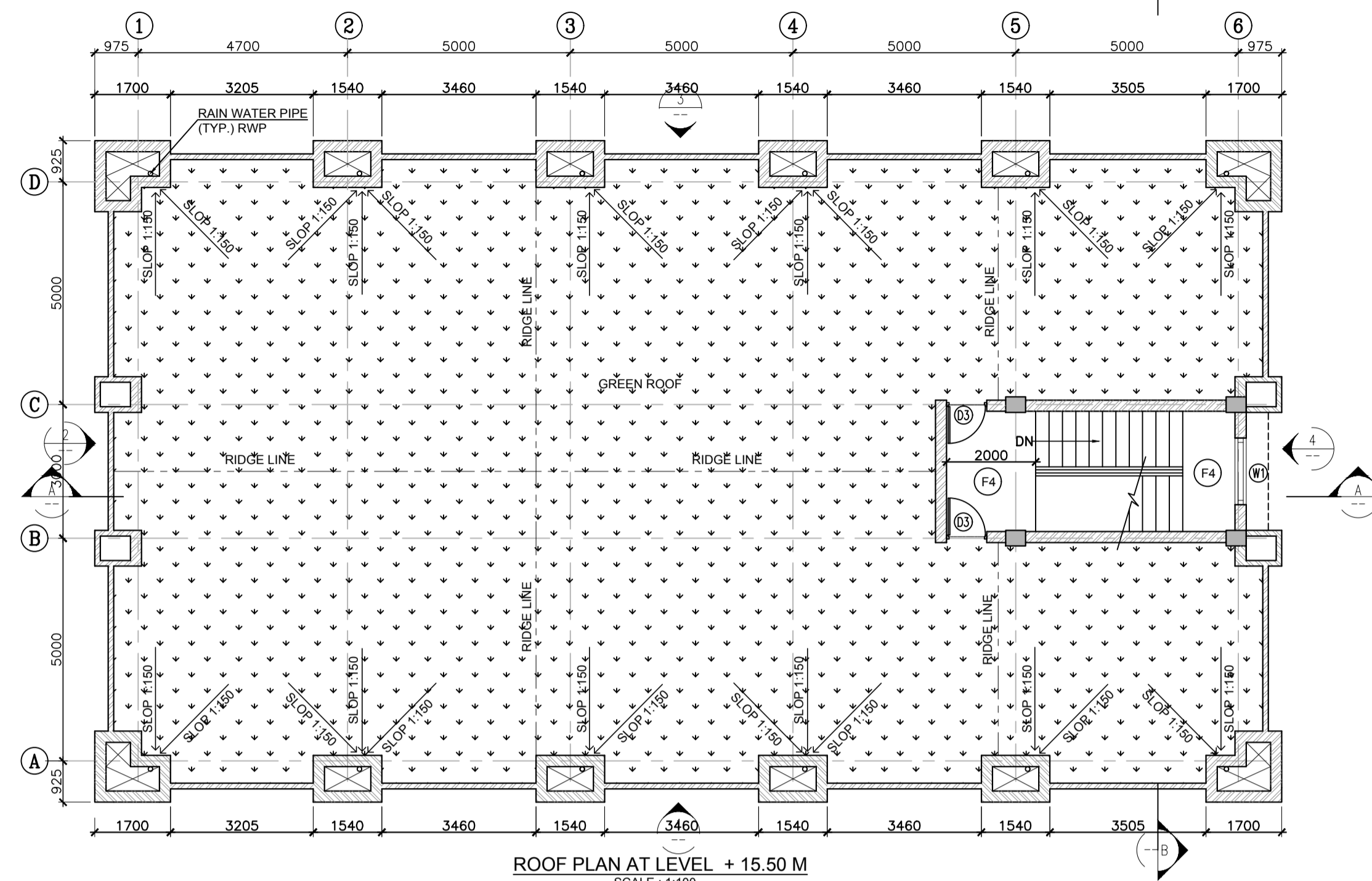
ROOF PLAN AT LEVEL + 15.50 M SCALE: 1:100
