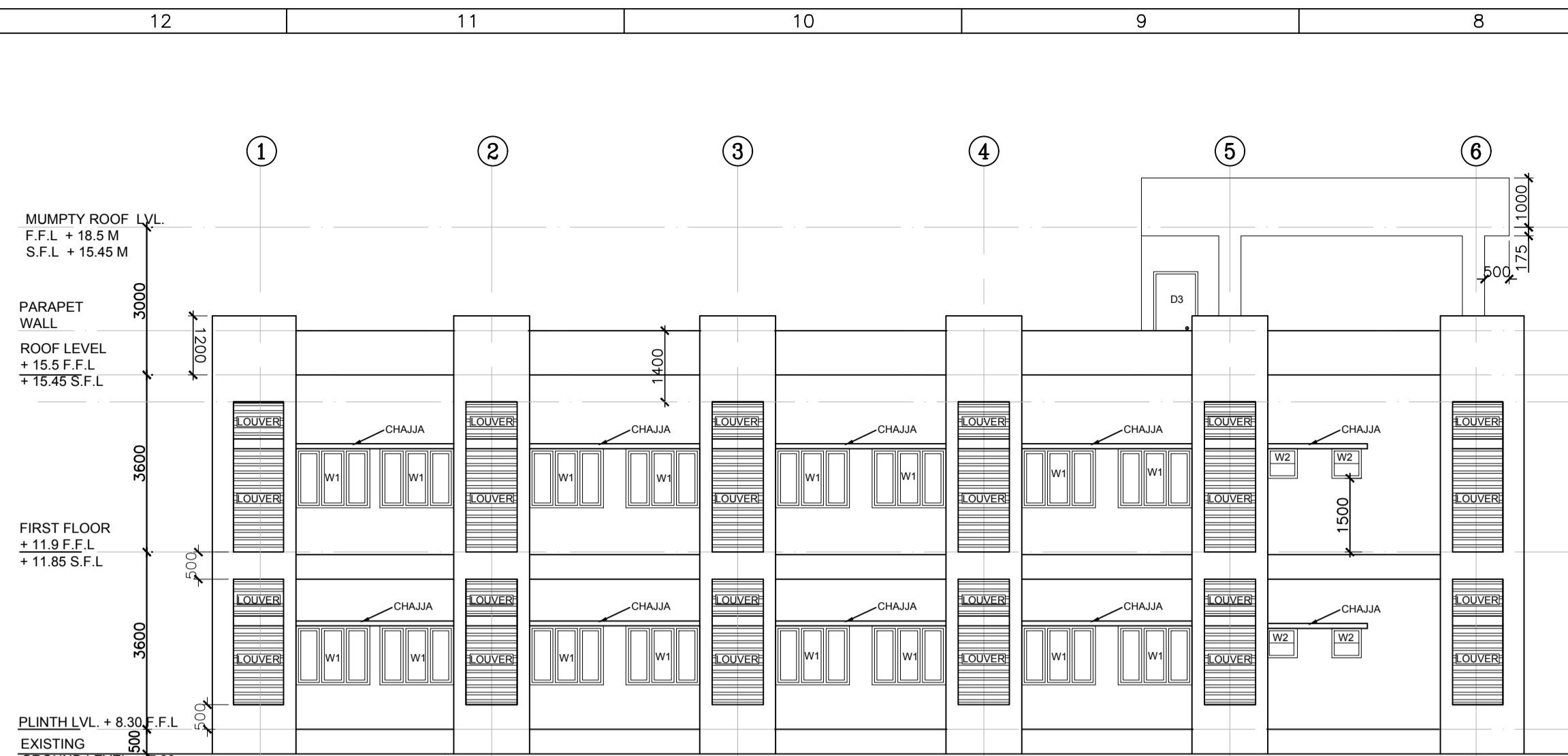
ELEVATION - 1 (SCALE 1:100)
