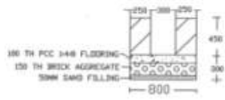
SECTION OF DRAIN E-E
