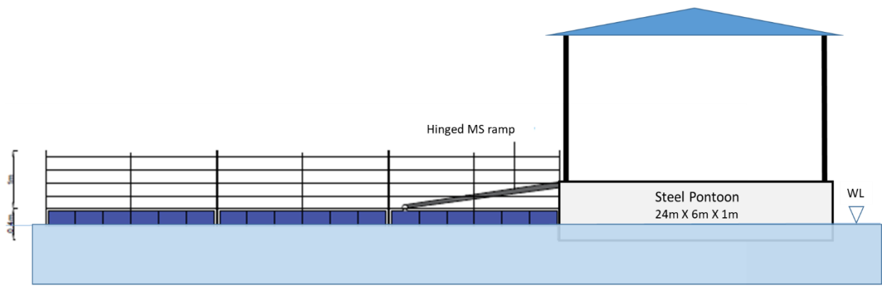
Proposed floating Gangway for Steel Pontoon
