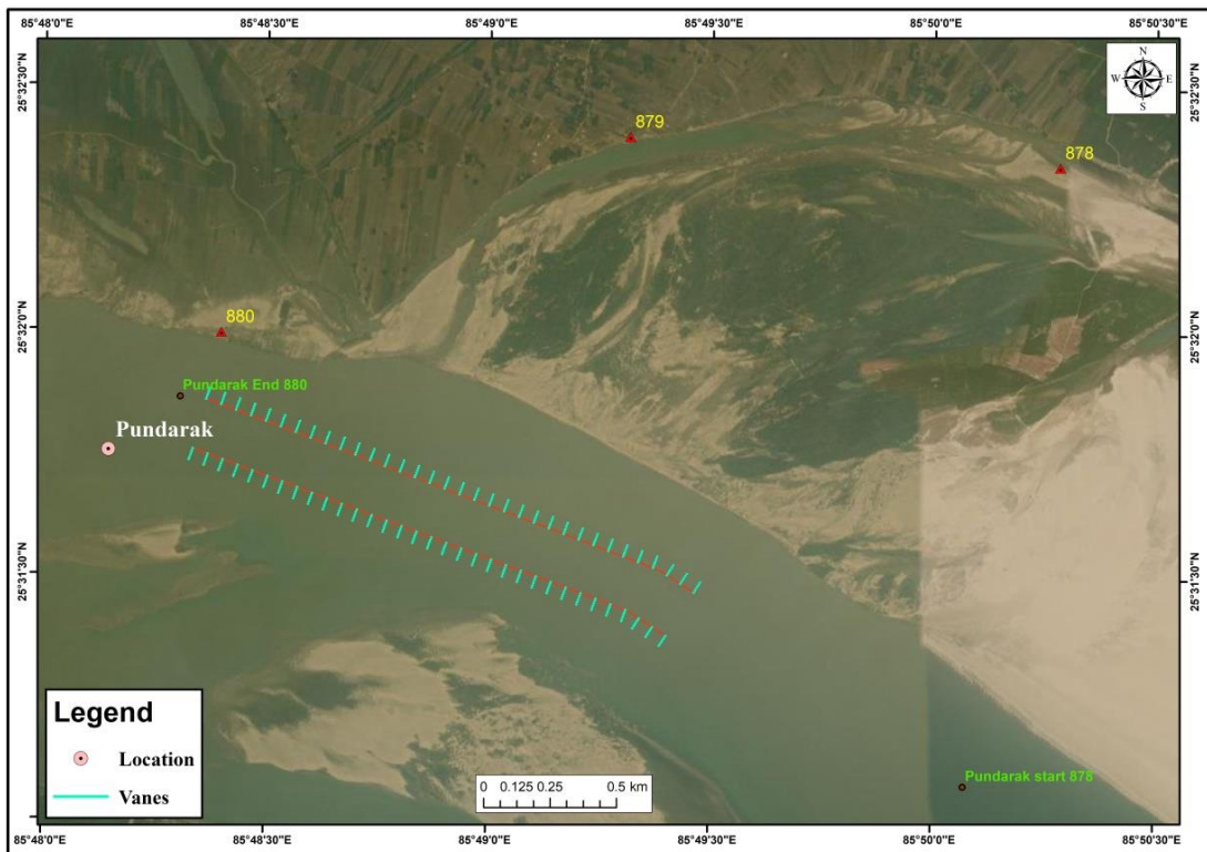
Proposed submerged vanes at Pundarak reach
