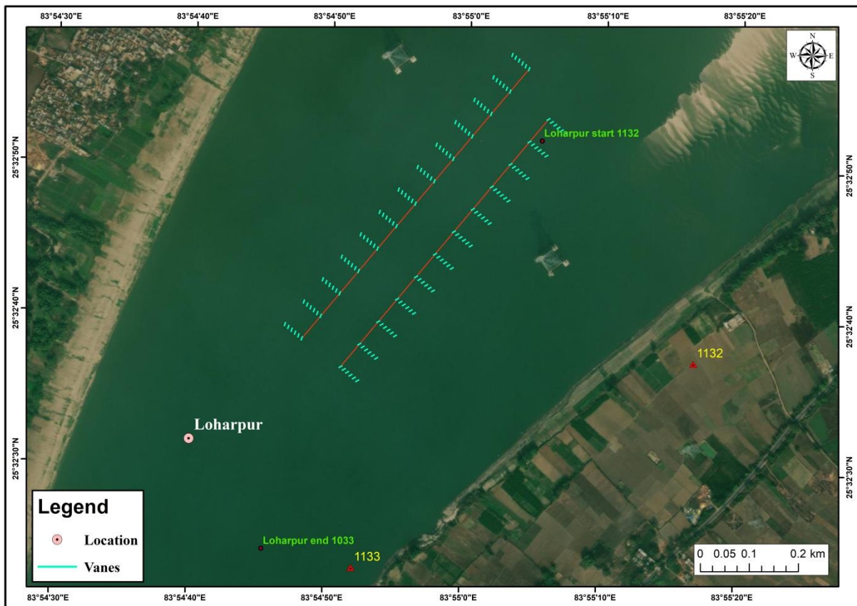
Proposed submerged vanes at Loharpur reach
