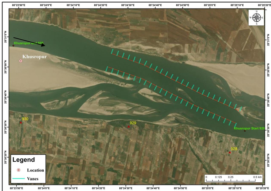
Proposed Submerged vanes at Khusropur reach
