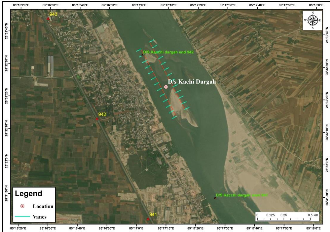
Proposed submerged vanes at Kachi Dargah reach
