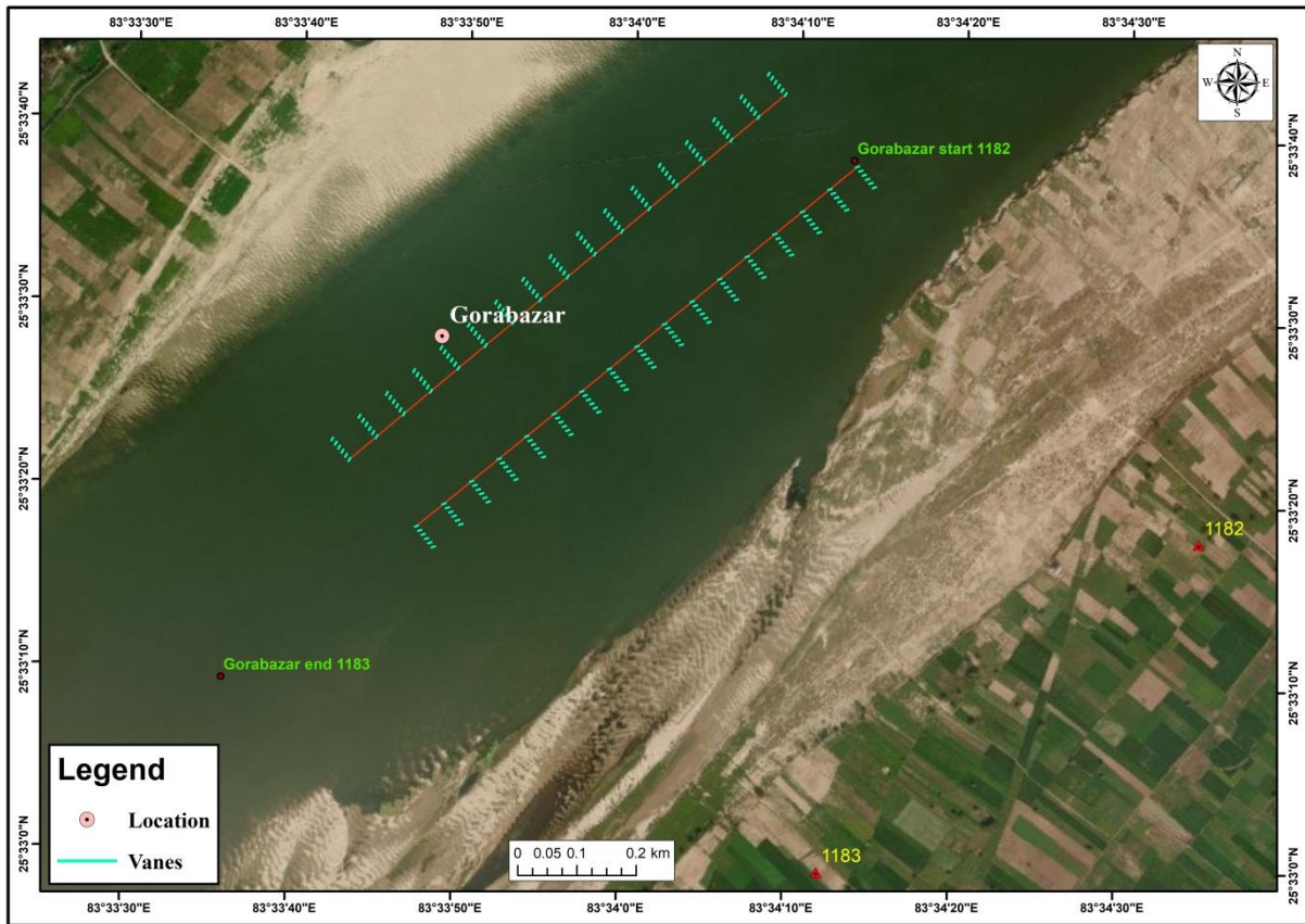
Proposed submerged vanes at Gorabazar
