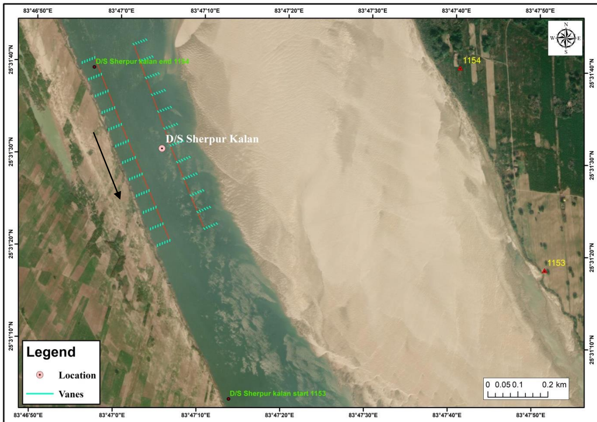
Proposed submerged vanes at Sherpur Kalan reach
