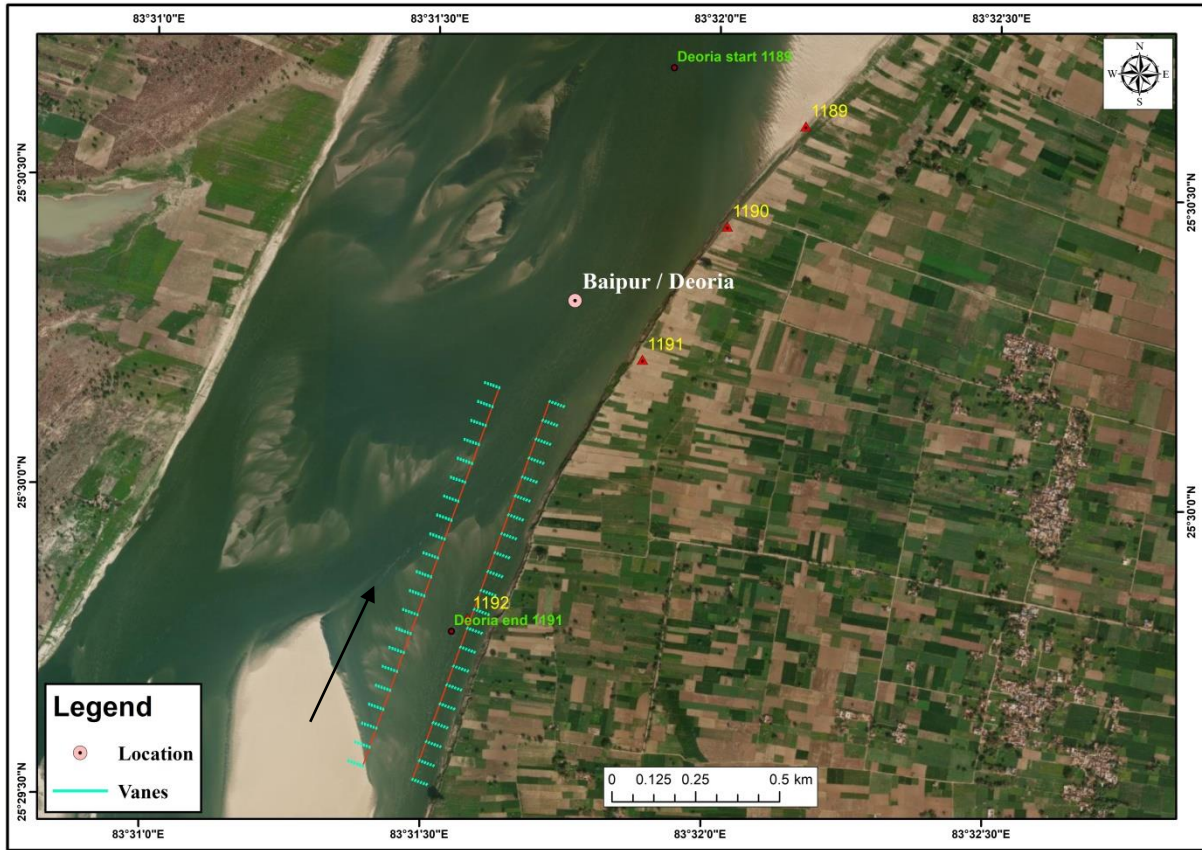
Proposed submerged vanes at Baipur reach
