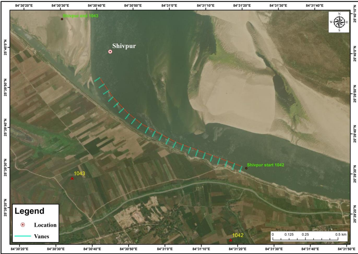
Proposed submerged vanes at Shivpur reach
