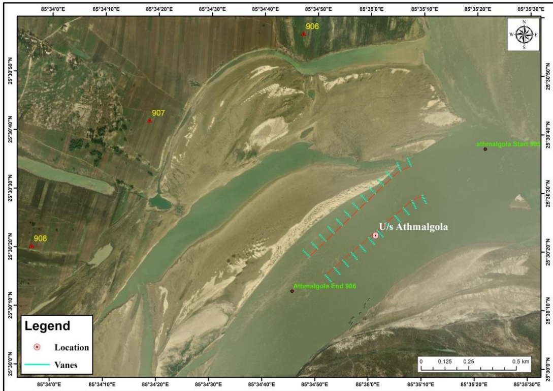
Proposed submerged vanes at Athmalgola reach
