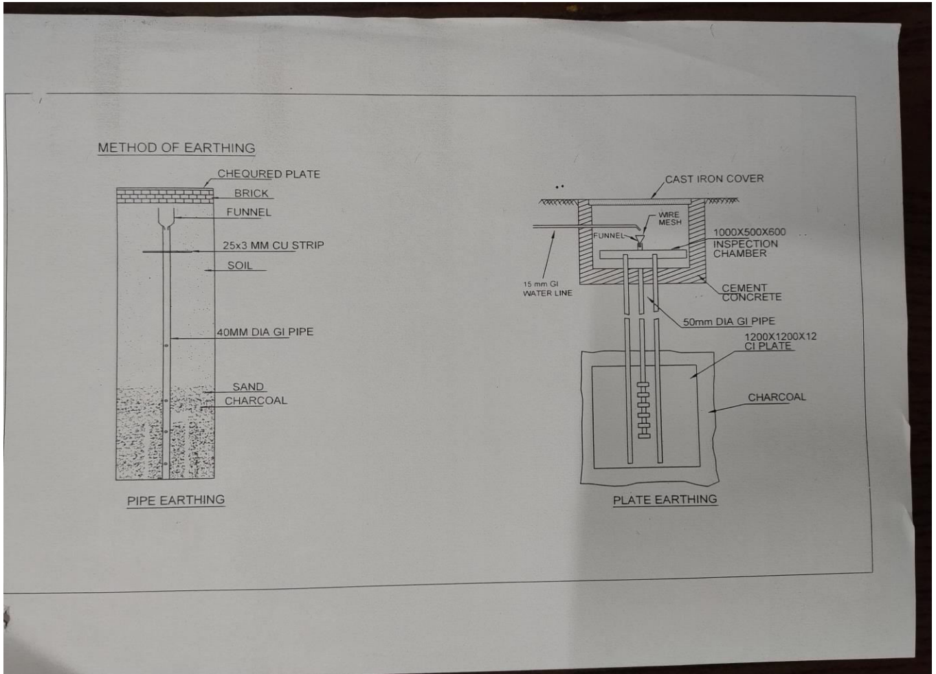
Fig: Drawing for installation of earthing point at Namoghat, Varanasi
