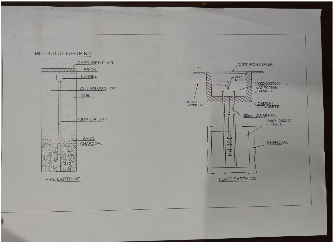
Fig: Drawing for installation of earthing point at Namoghat, Varanasi
