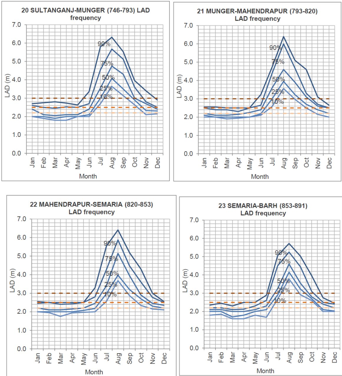
Figure A-2: Probability curves of LAD in Sultanganj-Barh
