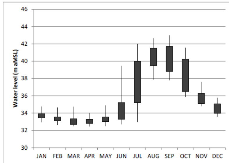
Figure A-1: Monthly water levels at Hathida (Chainage 850)
