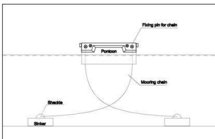
Fig 12. Typical chain mooring arrangement
