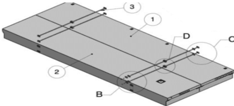
Fig 13. Side-by-side fixing arrangement
