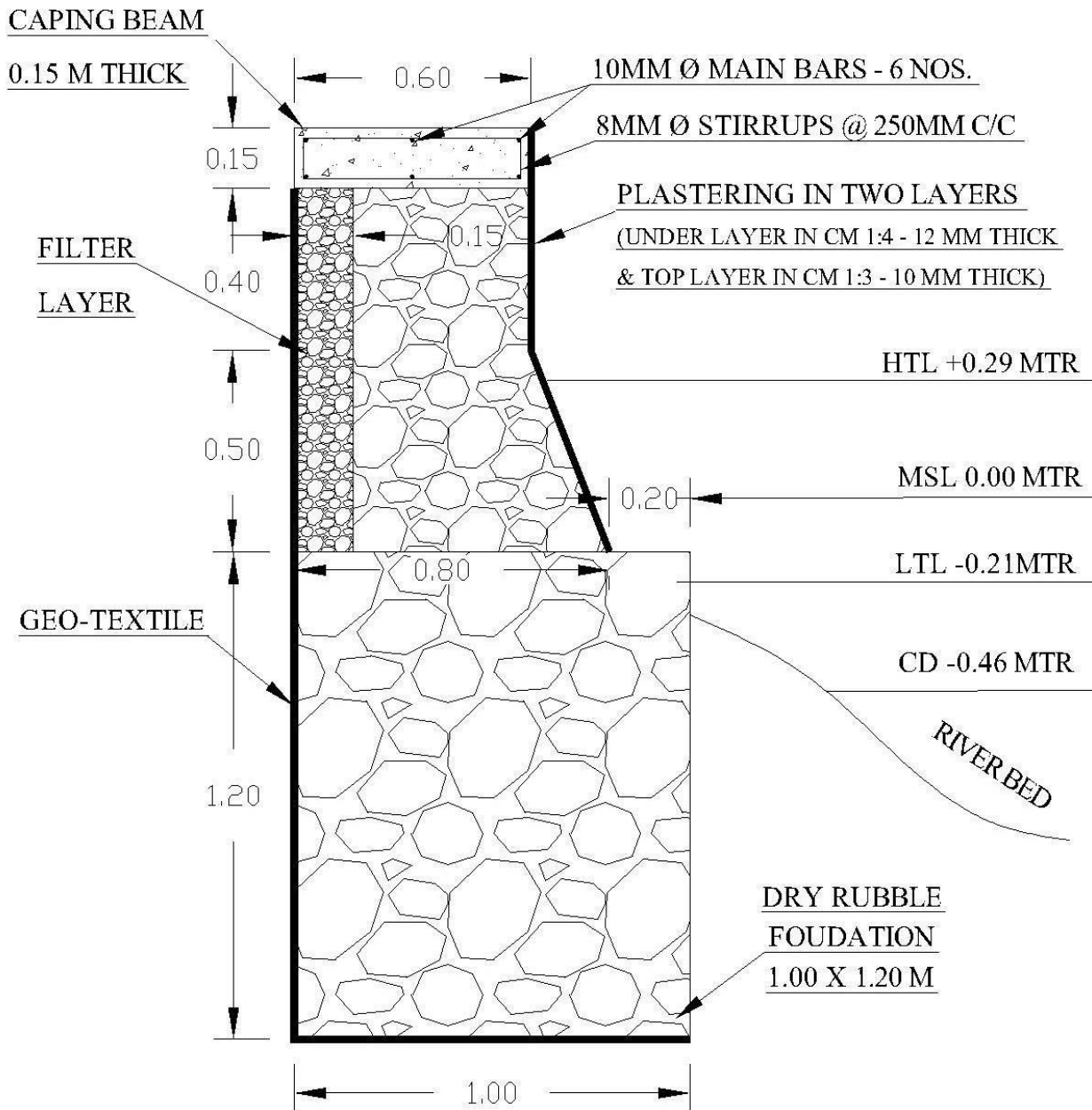
PROPOSED DESIGN FOR RIP-RAP TYPE BANK PROTECTION IN NW.3
