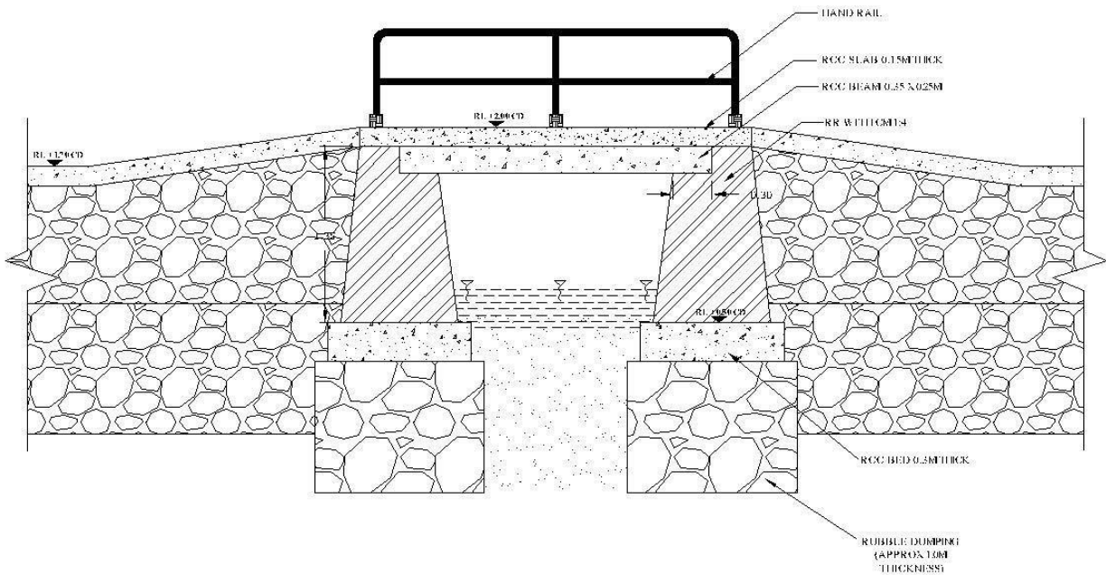
CROSS SECTION
