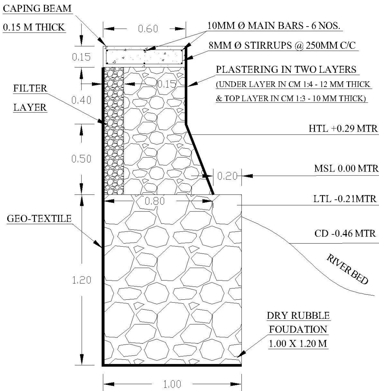
PROPOSED DESIGN FOR RIP-RAP TYPE BANK PROTECTION IN NW.3
