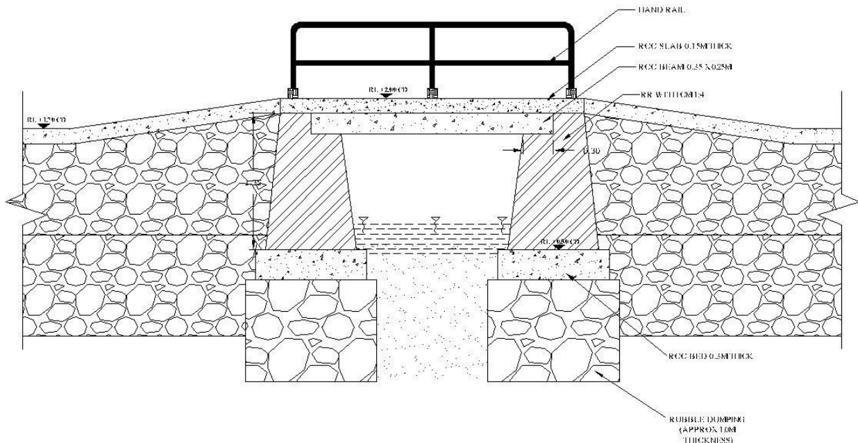
CROSS SECTION
