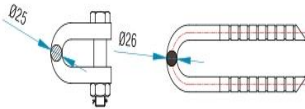
(3).D SHACKLE OF 25mm
