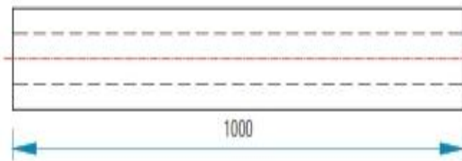
(1).CYC FENDER O.D.300XID.150 x 1 Mtr Lg.
