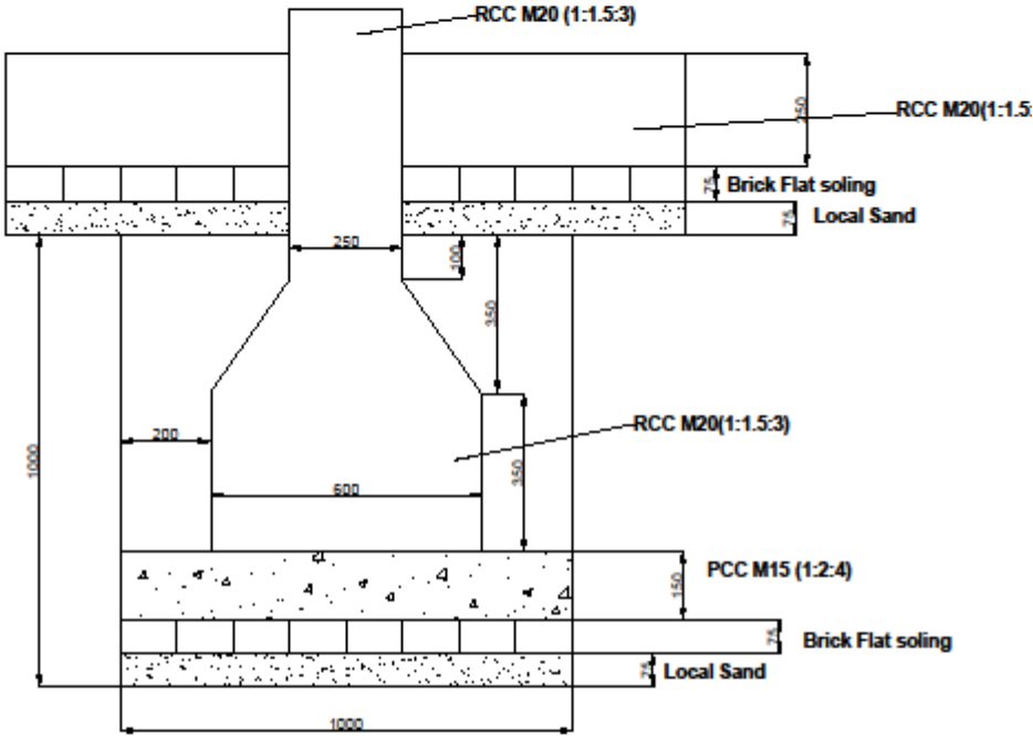
C/S FOOTING
