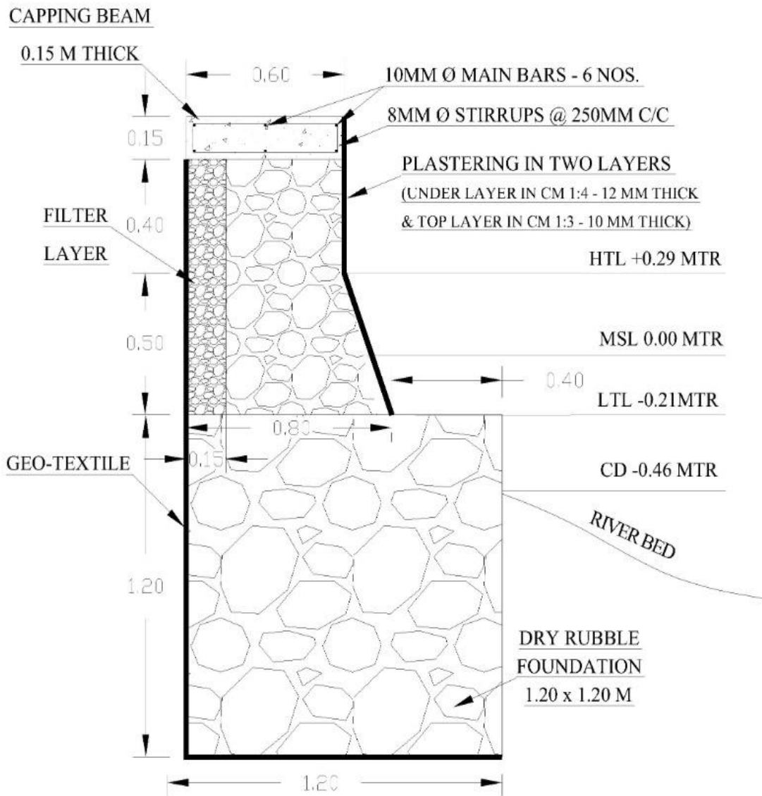
PROPOSED DESIGN FOR RIP - RAP TYPE BANK PROTECTION IN VARIOUS VULNERABLE LOCATIONS OF ALAPPUZHA - KODIMATHA STRETCH OF NW.9
