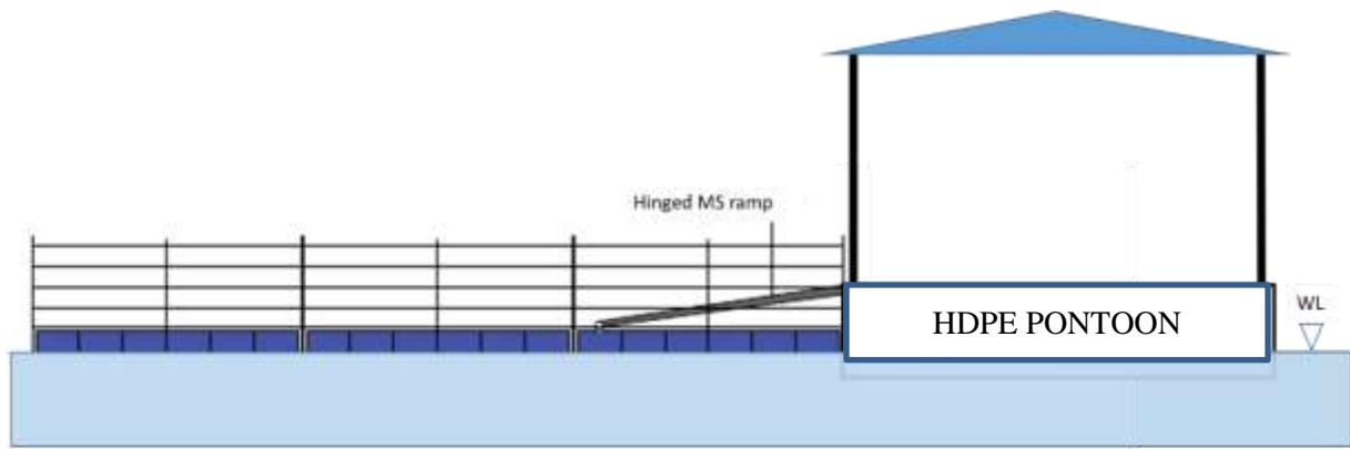
Proposed Floating Gangway for HDPE Pontoon
