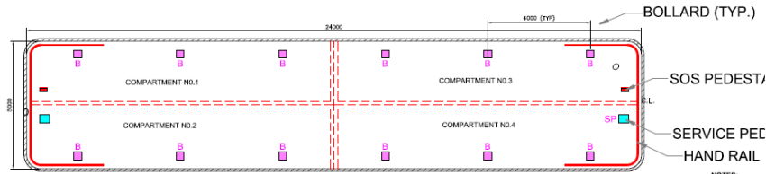
DECK PLAN - RCC PONTON
