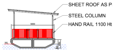
TYP. CROSS SECTION
