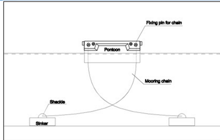
Fig 13. Typical chain mooring arrangement
