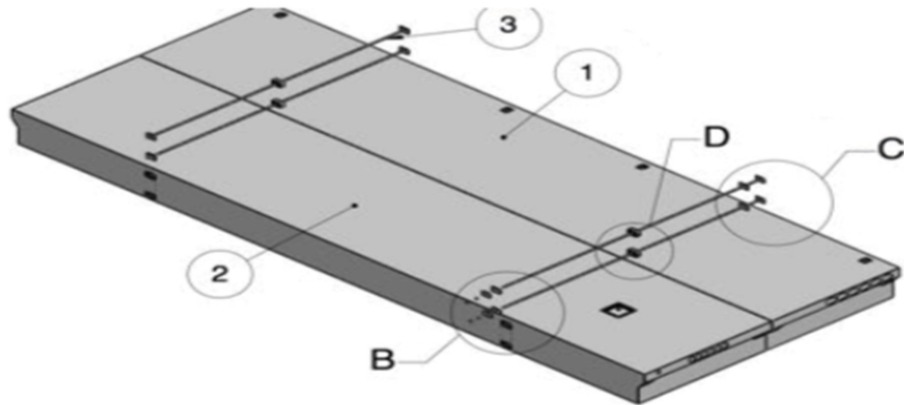
Fig 14. Side-by-side fixing arrangement
