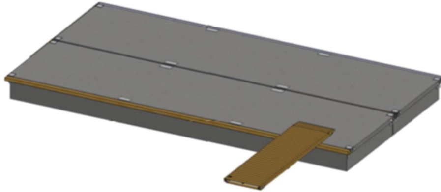
Fig 9 A 3-dimensional view of floating jetty arrangement with access gangway
