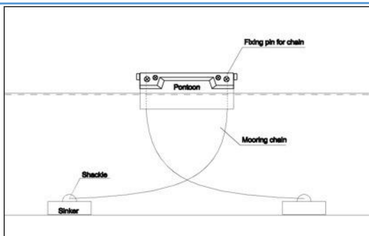
Fig 13. Typical chain mooring arrangement
