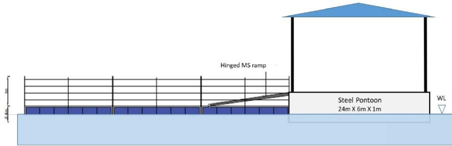
Proposed floating Gangway for Steel Pontoon
