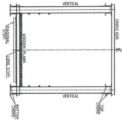
TRANSV. SECTION THROUGH VERTICAL MEMBERS
