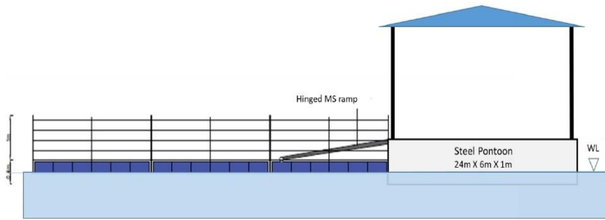
Proposed floating Gangway for Steel Pontoon
