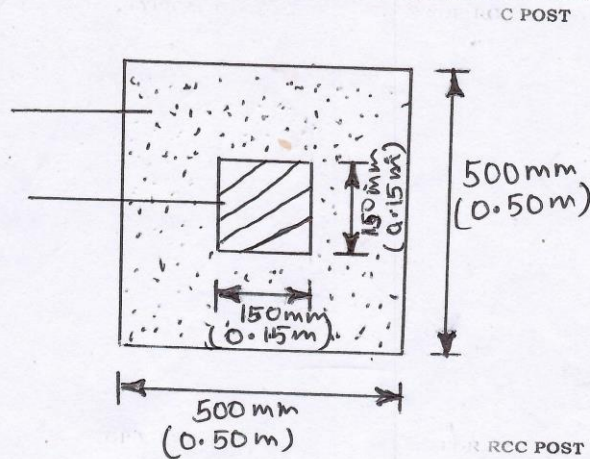
TOP VIEW OF FOUNDATION DETAIL FOR RCC POST
