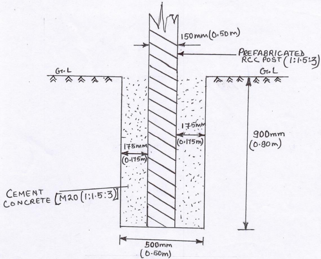
TYPICAL C/S OF FOUNDATION FOR RCC POST
